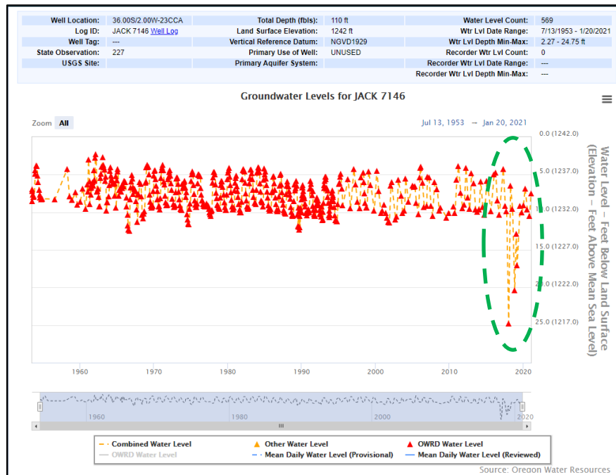
Figure 5.8: Well JACK 7146
